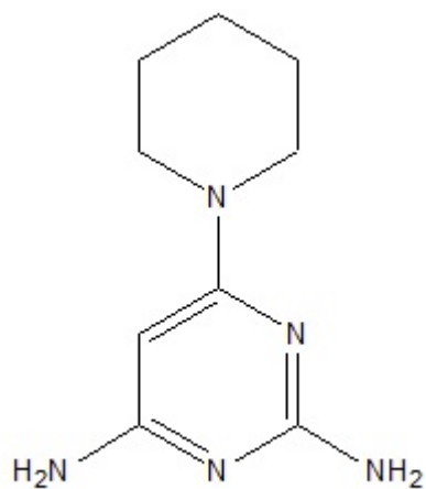
2,4-Diamino-6-piperidinopyrimidine
