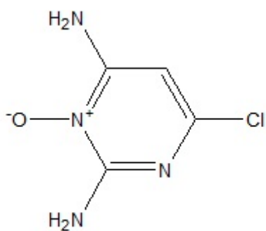
2,4-Diamino-6-chloropyrimidine-3-oxide
