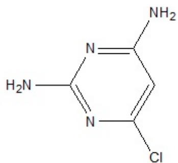
2,4-Diamino-6-chloropyrimidine
