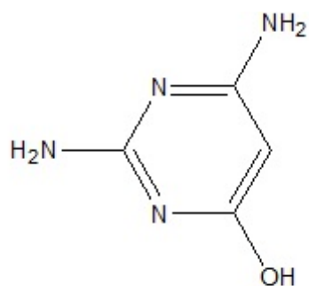
2,4-Diamino-6-hydroxypyrimidine
